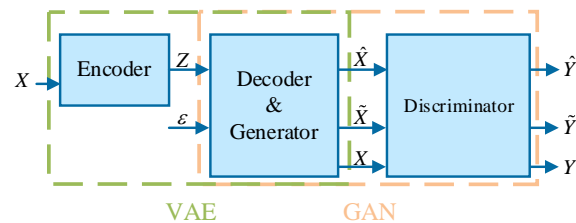
Fig. 1. Structure of VAEGAN.
