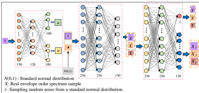
Fig. 3. Structure of Enhanced VAEGAN model.
